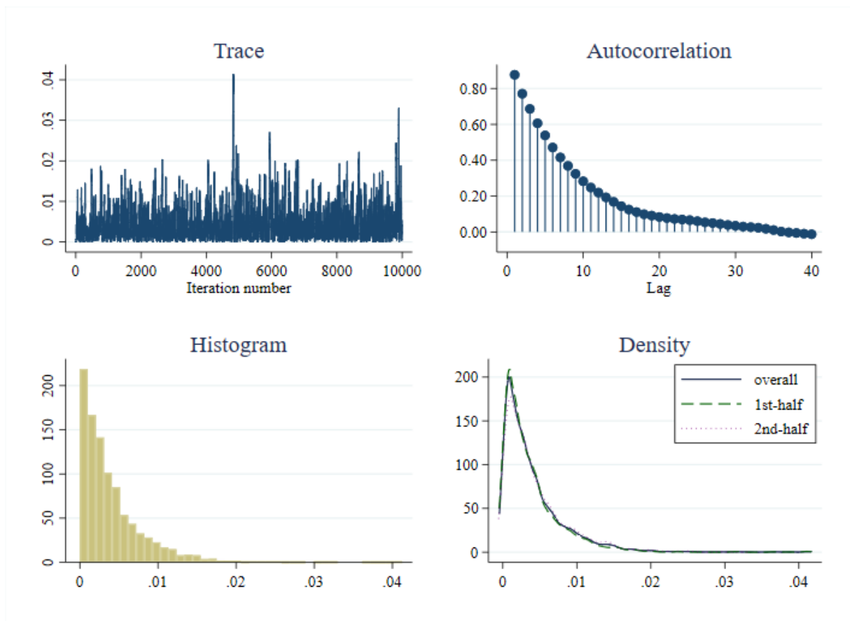
Figure 4: Intra-temporal substitution
