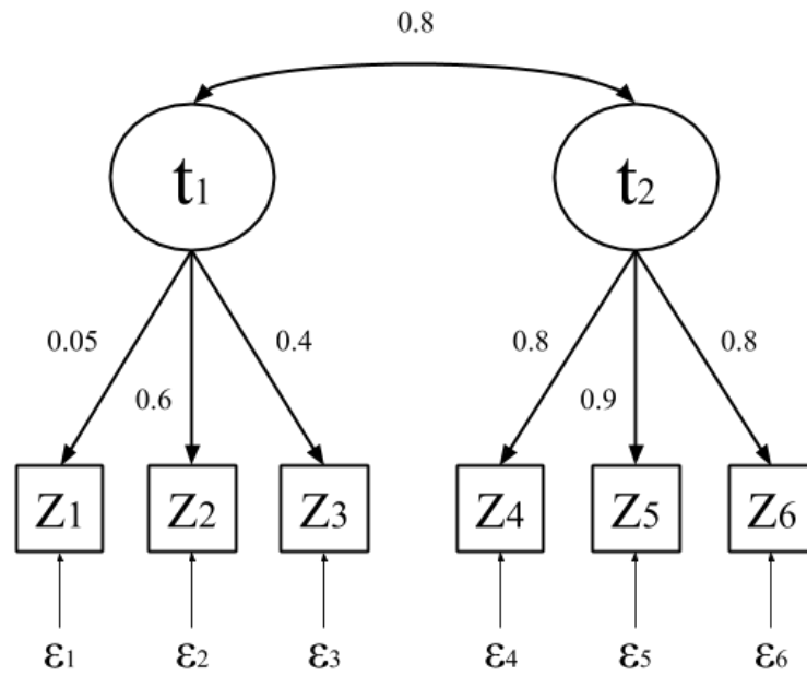
Figure 3: The problem of a small factor loading and a large correlation
